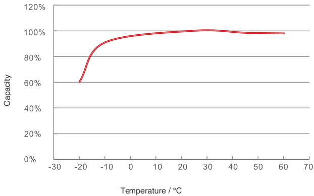
Different Temperature Self Discharge Curved
