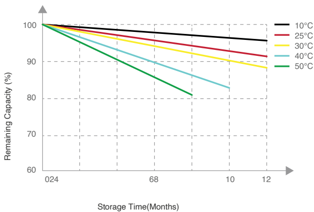
Different Temperature Self Discharge Curved
