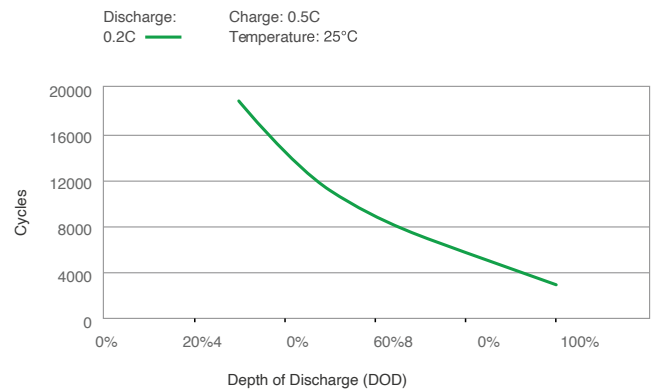
ifferent DOD Discharge Cycle Life Curve
